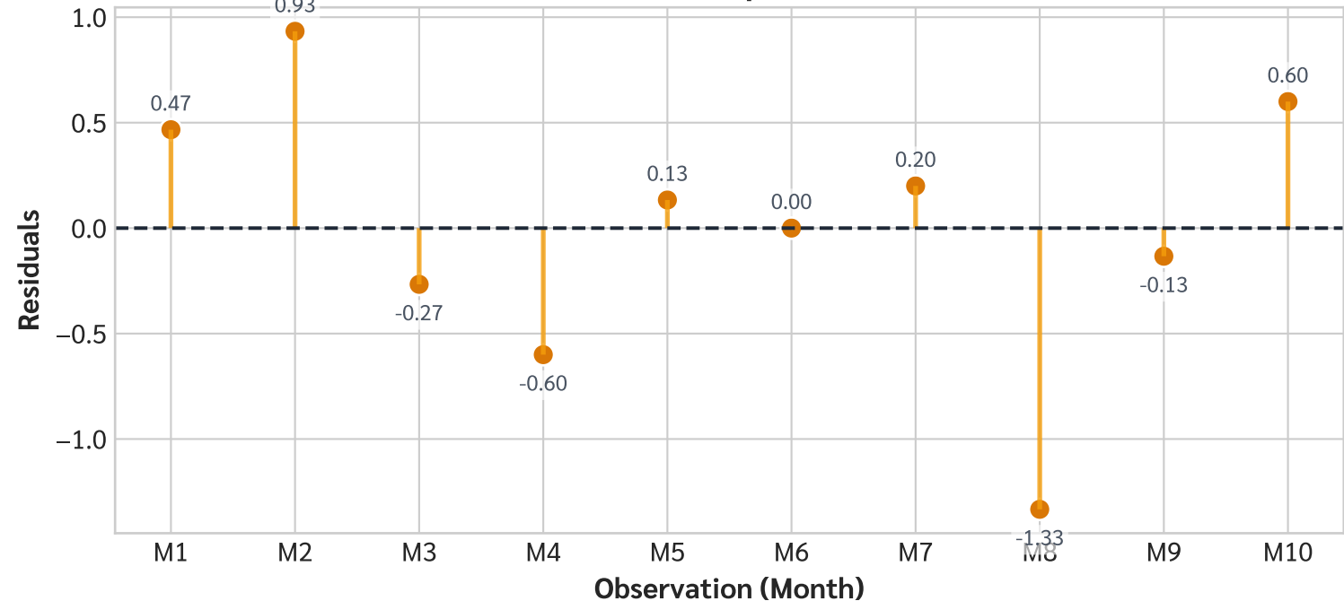
Residuals (Errors) per Observation
